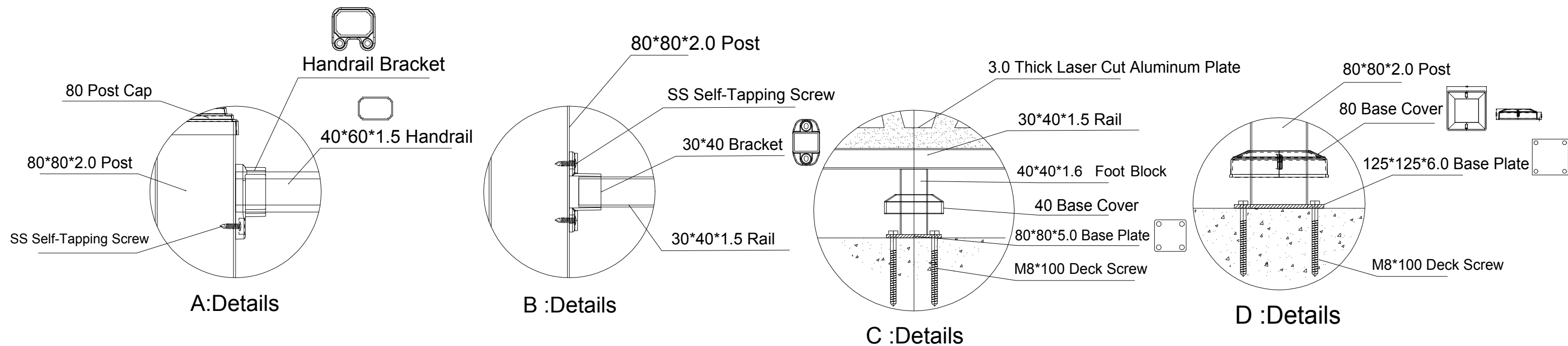
Sectional Drawing
