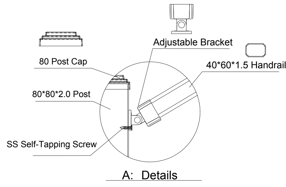
Sectional Drawing
