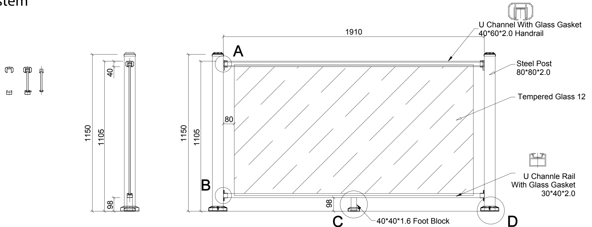
Sectional Drawing
