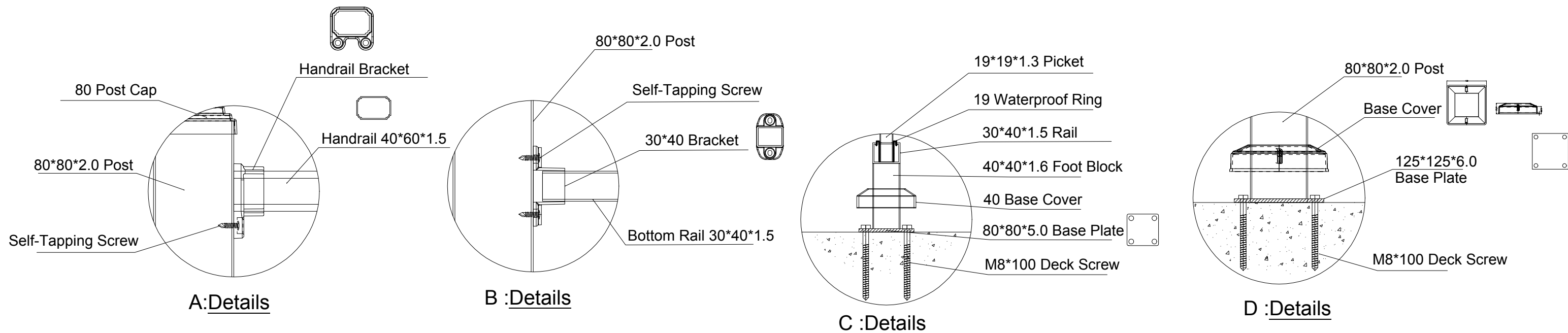
Sectional Drawing
